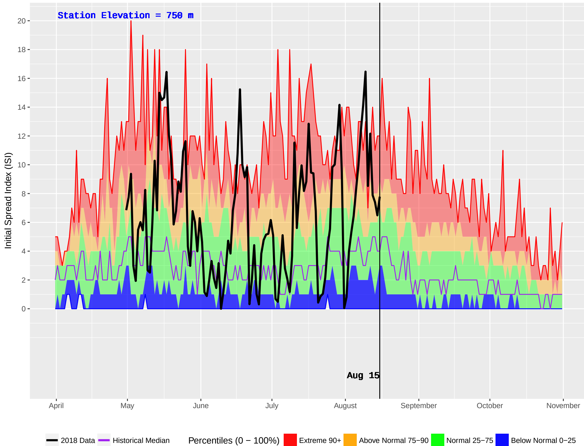
FORT ST JAMES (146) : Historical (1979–2016) and Current (2018) Daily Initial Spread Index (ISI)
