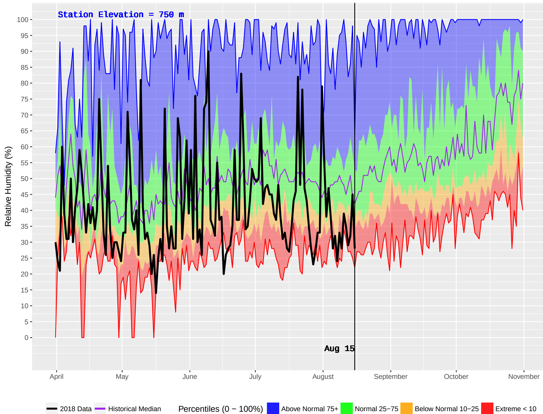
FORT ST JAMES (146) : Historical (1979–2016) and Current (2018) Daily Relative Humidity
