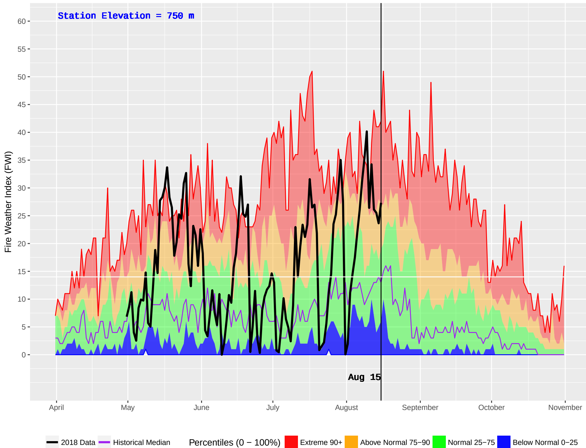
FORT ST JAMES (146) : Historical (1979–2016) and Current (2018) Daily Fire Weather Index (FWI)
